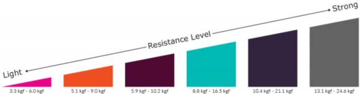
Typical Pull Force Chart With An Elongation Percentage of 100% to 300%
